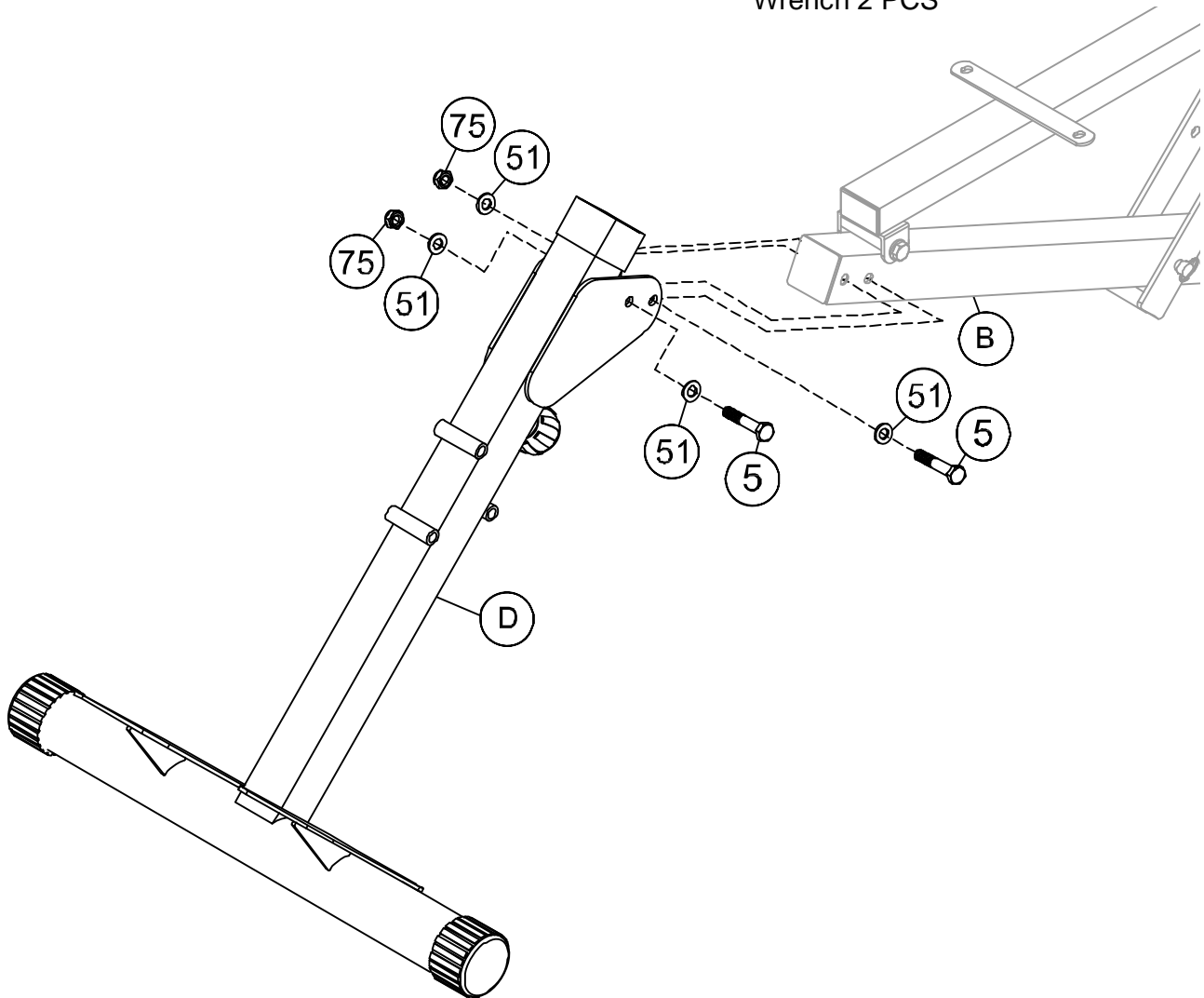
Wrench 2 PCS
